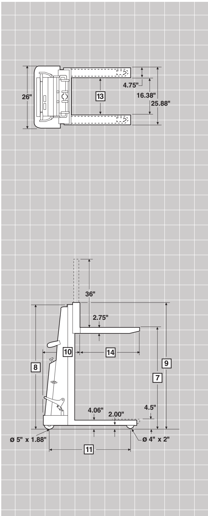
Model 20B Fork Over
